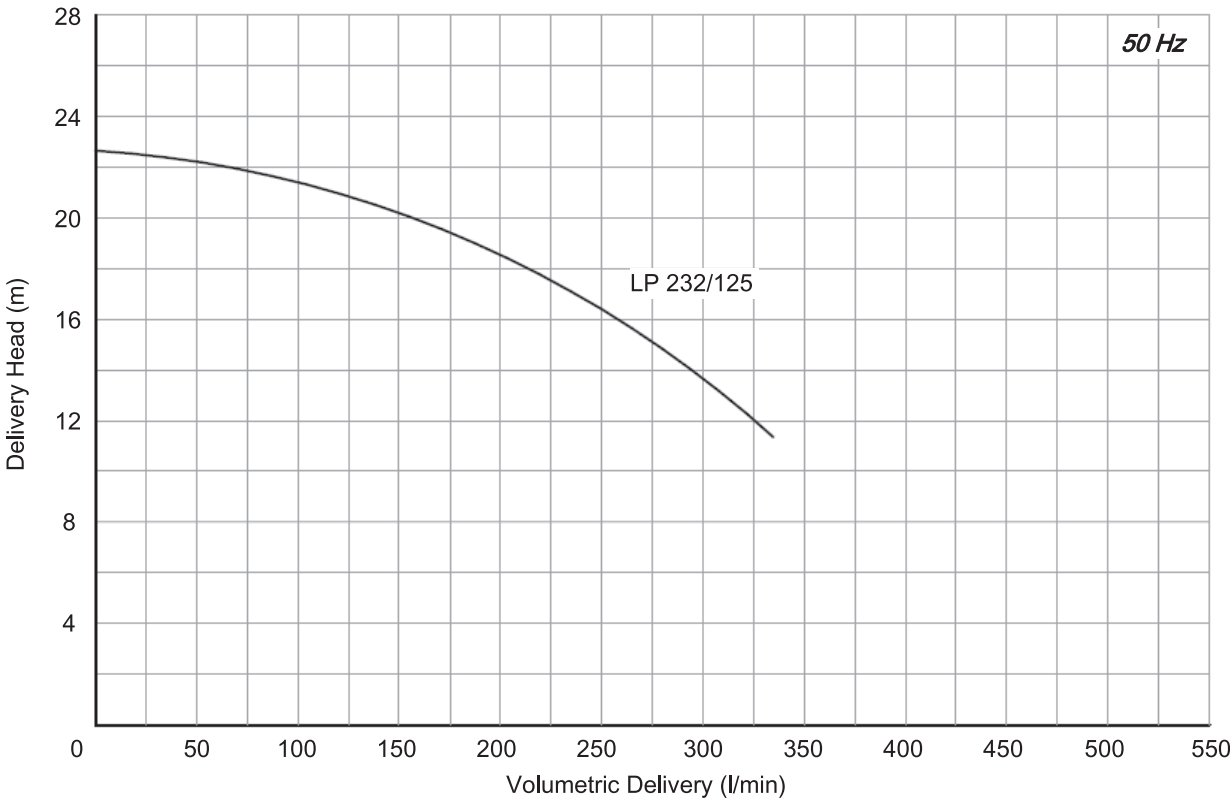
Performance Curve
