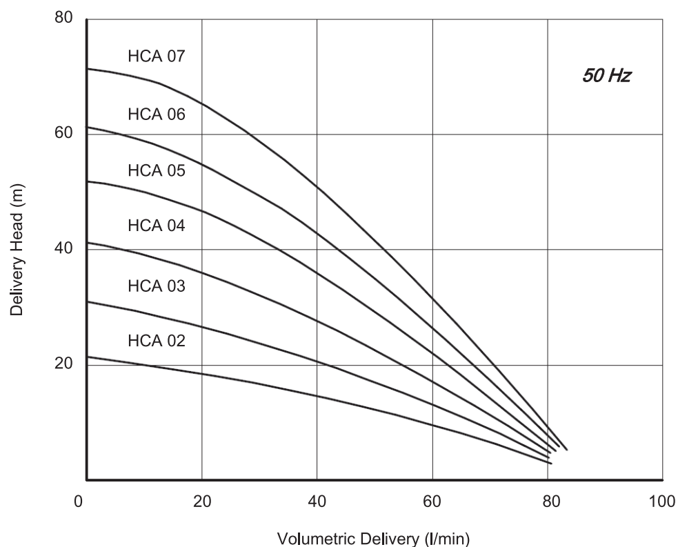
Performance Curve
