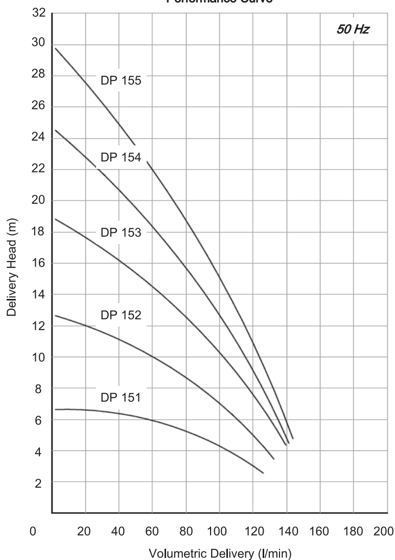
Performance Curve
