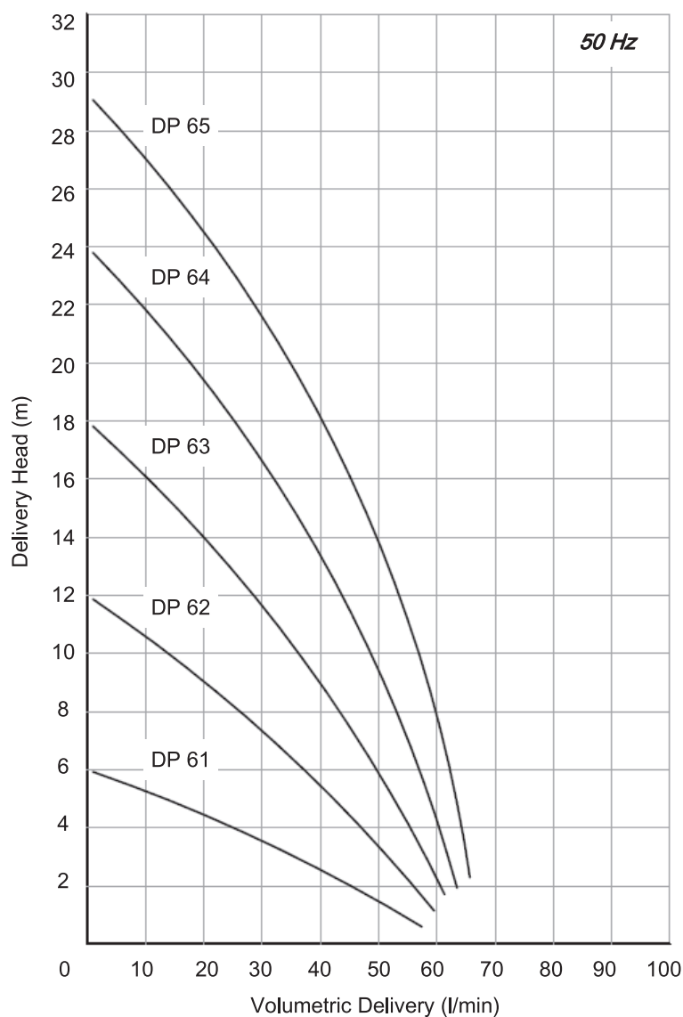
Performance Curve
