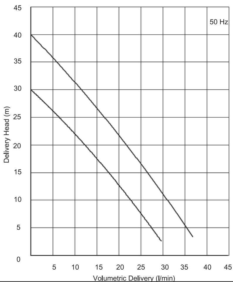
Performance Curve
