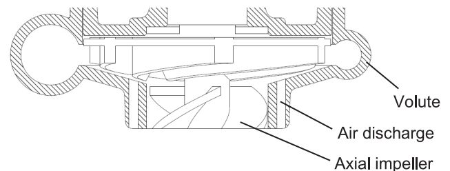
JB H 350 - Axial front impeller with air release
