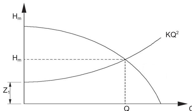
Figure 11 - Determining of the operating point
